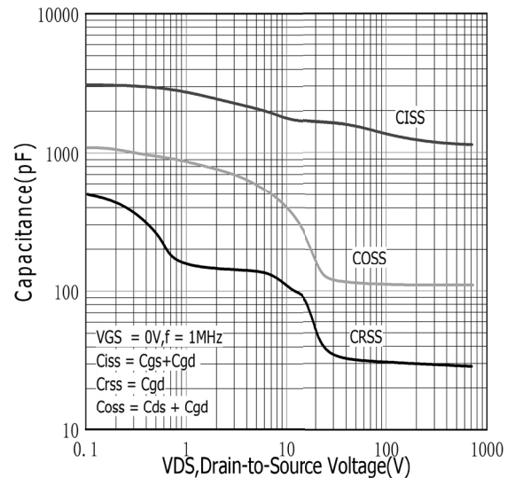
Figure.4 Typical Capacitance vs Drain to Source Voltage
